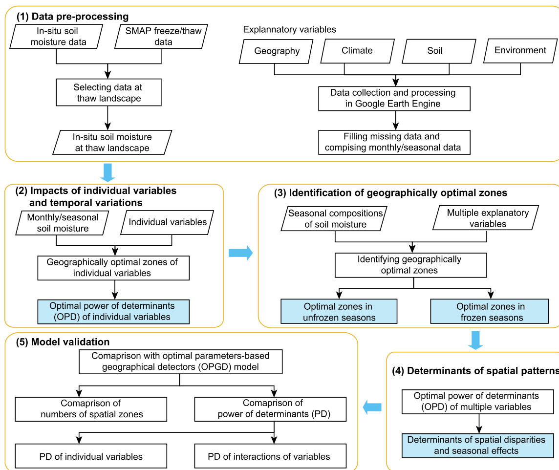
Fig. 2. Schematic overview of GOZH -based identification of determinants for spatiotemporal heterogeneity of soil moisture in the Northern Hemisphere.
